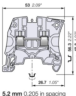
5.2 mm 0.205 in spacing
