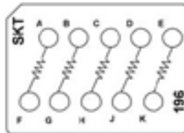
CTJ420E196 Five 127 \Omega Resistors, 1/8 W
