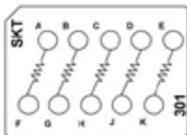
CTJ420E301 Four 2.7 k \Omega Resistors, 1/4 W One 56 \Omega Resistor, 1/2 W
