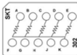
CTJ420E302 Four 2.7 k \Omega Resistors, 1/4 W One 3.9 k \Omega Resistor, 1/4 W
