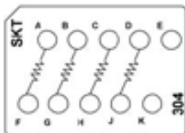
CTJ420E304 Two 120 \Omega Resistors, 1/2 W Two 2.7 k \Omega Resistors, 1/4 W
