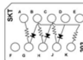
CTJ420E303 One 2.7 k \Omega Resistor, 1/4 W One 1.8 k \Omega Resistor, 1/4 W One 5.1 k \Omega Resistor, 1/4 W One 3.3 k \Omega Resistor, 1/4 W Three JANTX 1N5711 Diodes
