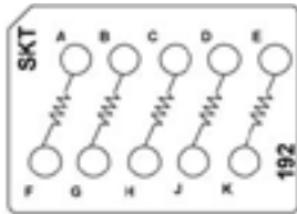
CTJ420E192 Five 1 k \Omega Resistors, 1/4 W
