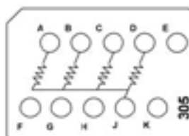
CTJ420E305 Two 2.7 k \Omega Resistors, 1/4 W Two 3.9 k \Omega Resistors, 1/4 W
