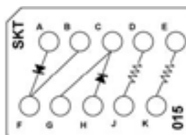
CTJ420E015 Two JANTX 1N5618 Diodes One 10 k \Omega Resistor, 1/10 W One 110 \Omega Resistor, 1/10 W
