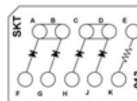
CTJ420E013 Four JANTX 1N5618 Diodes One 200 \Omega Resistor, 1/8 W
