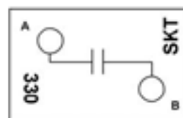
CTJ420E330 One 1000 pF Capacitor, 100 VDC
