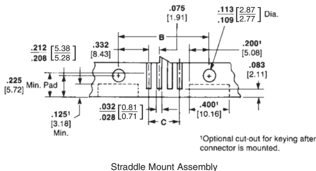
Straddle Mount Assembly
