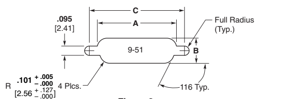
Figure 2 Rear Mounting
