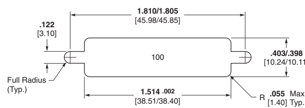
Rear Mounting
