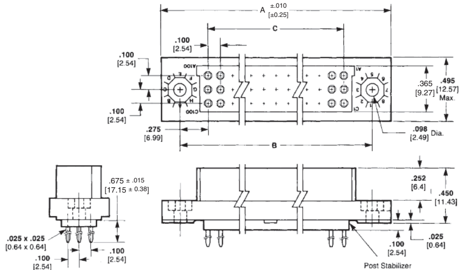
Wrap-Type Posted Contact
