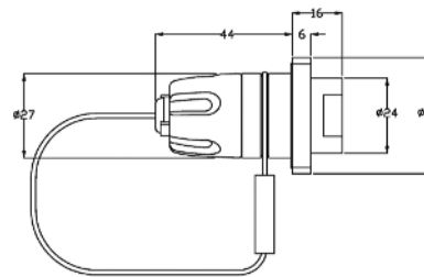
PRO BEAM Jr., Low Profile, Square Flange Mount Bulkhead Connector
