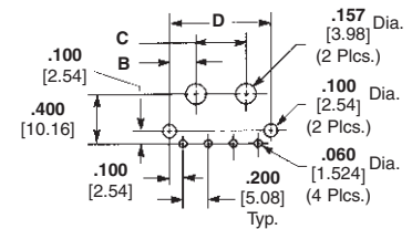
Recommended PC Board Hole Layout .062 [1.57] thick PC Board
