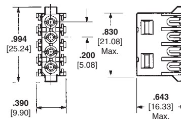
Socket Assembly (Plug)
