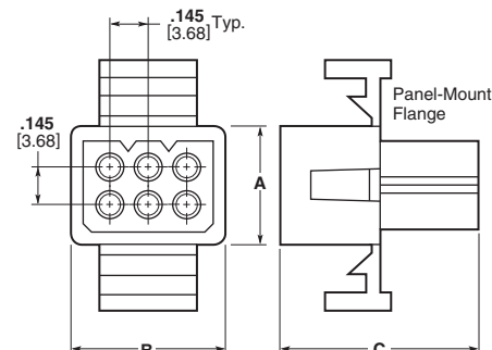
Plug
