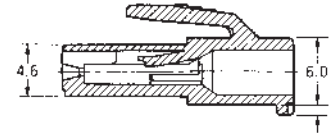
Section X-X
