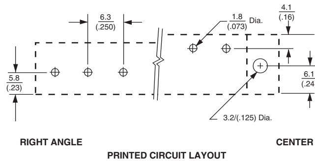
PRINTED CIRCUIT LAYOUT
