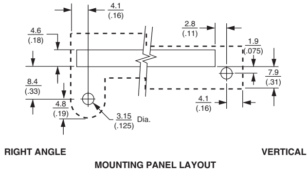
MOUNTING PANEL LAYOUT
