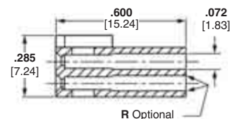
Section X-X
