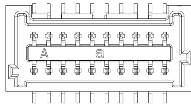
20 POSITION 2-2456589-0
