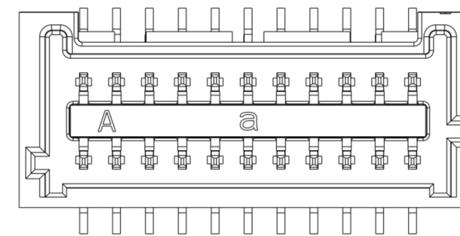
22 POSITION 2-2456589-2
