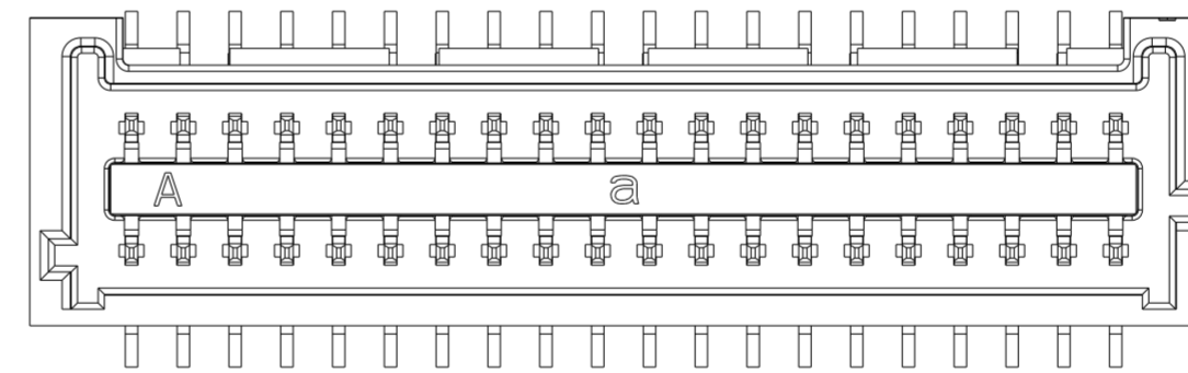
40 POSITION 4-2456589-0
