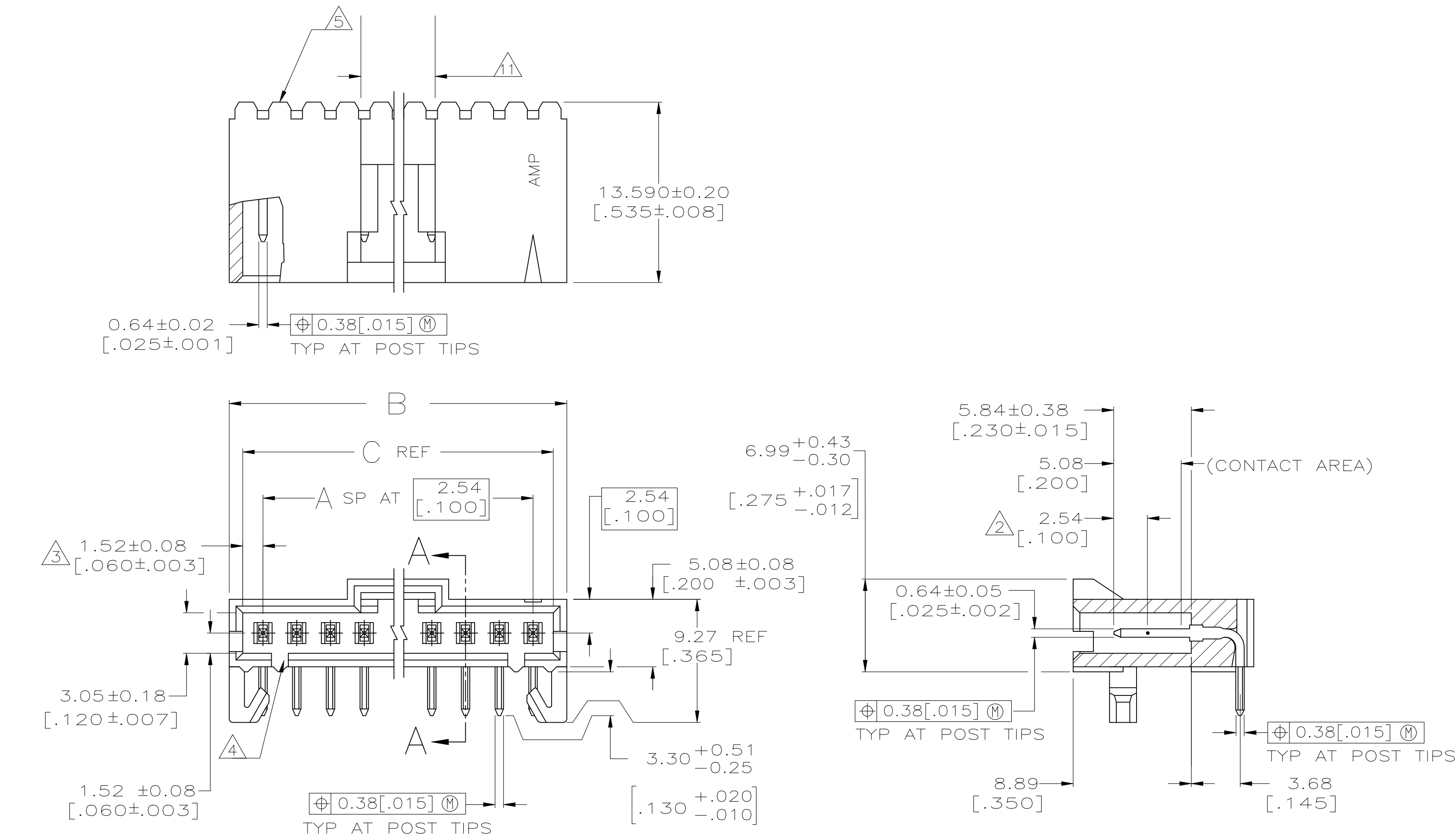
SECTION A—A
