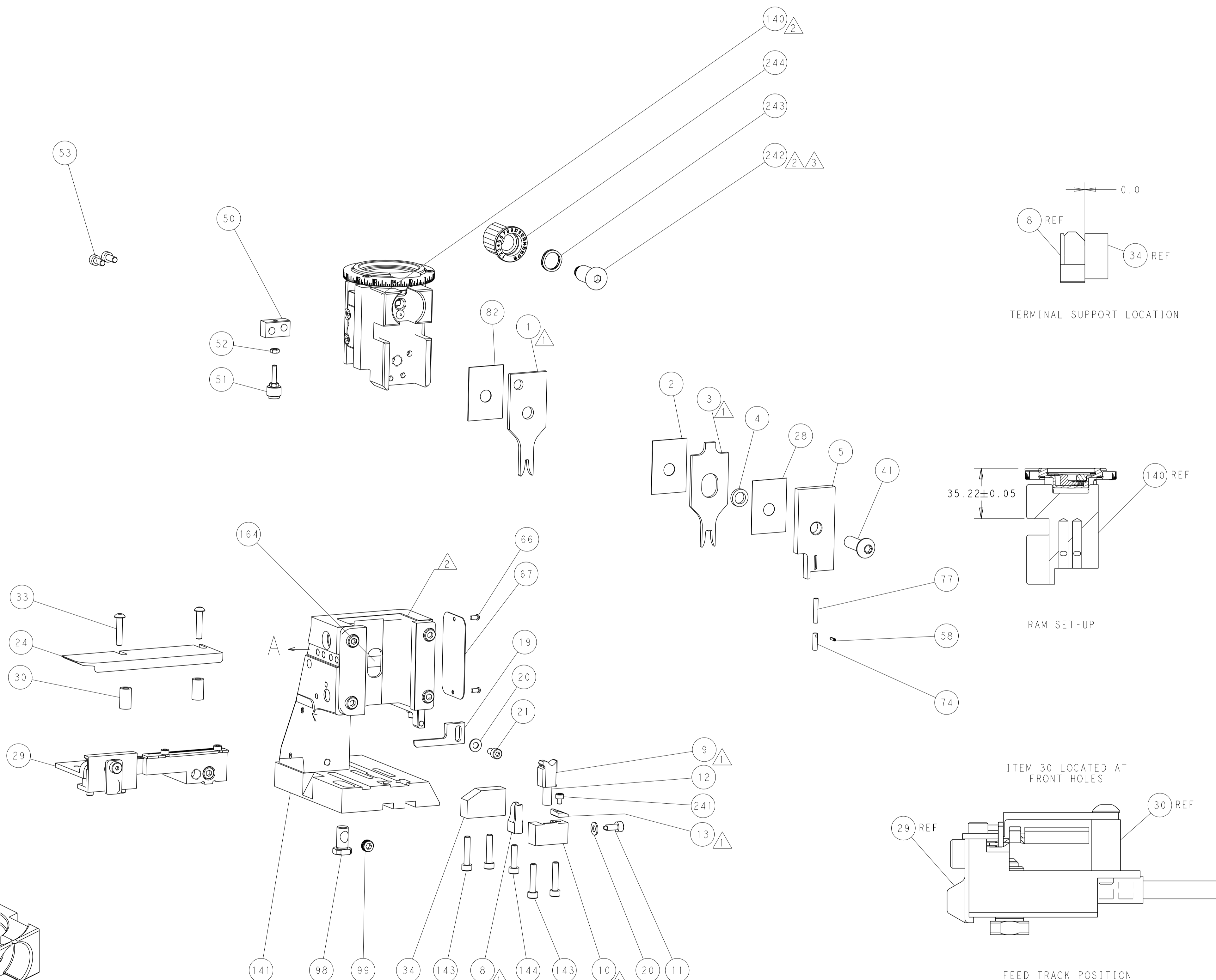
FEED TRACK POSITION GUIDE BY INSULATION BARREL
