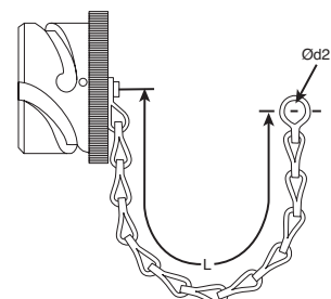
CIRB-**-E-PCAK (with sash chain)
