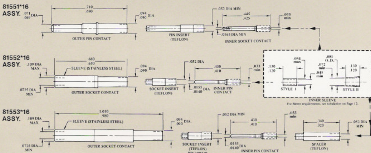
CONTACT ASSEMBLY SPECIFICATIONS
