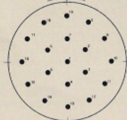
J04(2419) 19 NO. 12 CONTACTS
