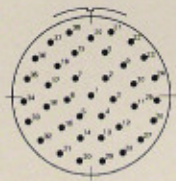
F02(1838) 38 NO. 20 CONTACTS
