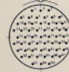
E01(1655) 55 NO. 23 CONTACTS
