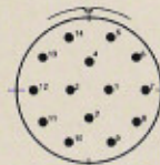
E03(1614) 14 NO. 16 CONTACTS
