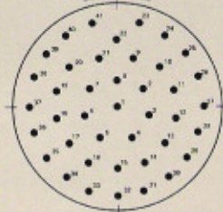
J03(2441) 41 NO. 16 CONTACTS
