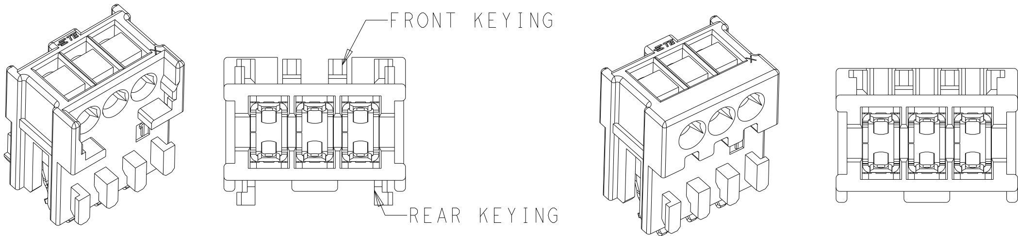
OPTION A FRONT KEYING + REAR KEYING OPENING ON FRONT OPTION B FRONT KEYING ONLY CLOSING ON FRONT
