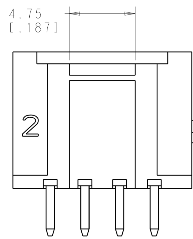
SINGLE LATCH DETAIL 1969582-8 SHOWN HERE THESE DIM'S ARE FOR THE 1969582-8 AND 1-1969582-0
