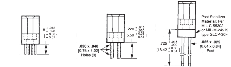
.014 x .019 [0.36 x 0.48] Channel Contact
