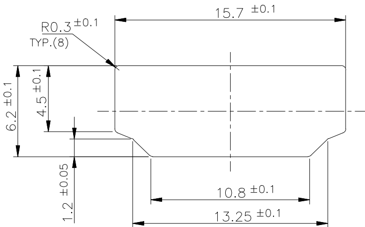
PANEL CUT OUT DIMENSION (REFERENCE)
