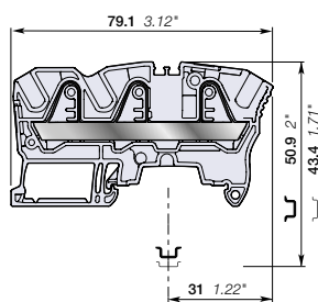
ZK6-3P
