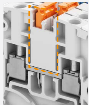
Closed jumper location for stiffness
