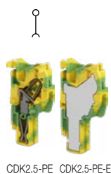
CDK2.5-PE CDK2.5-PE-E
