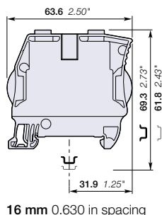
16 mm 0.630 in spacing
