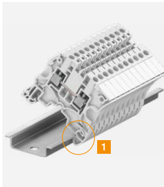
Lock up to ten blocks in position at a time
