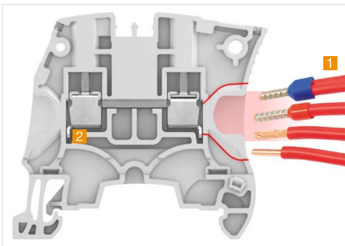
Engineered conductor entry
