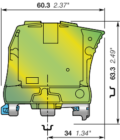
32 mm 1.260 in spacing
