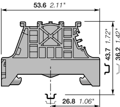
BAM4
