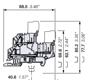
7DK2.5-D2-PF
