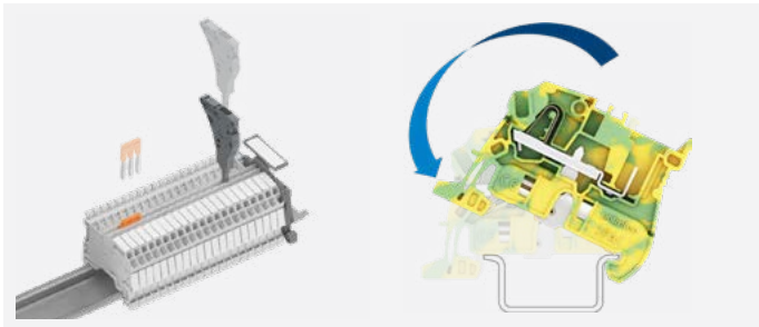
Screwless accessories
