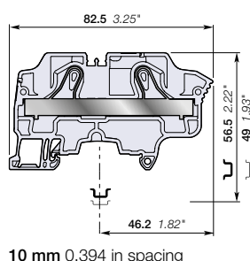
10 mm 0.394 in spacing
