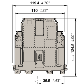
36 mm 1.417 in spacing
