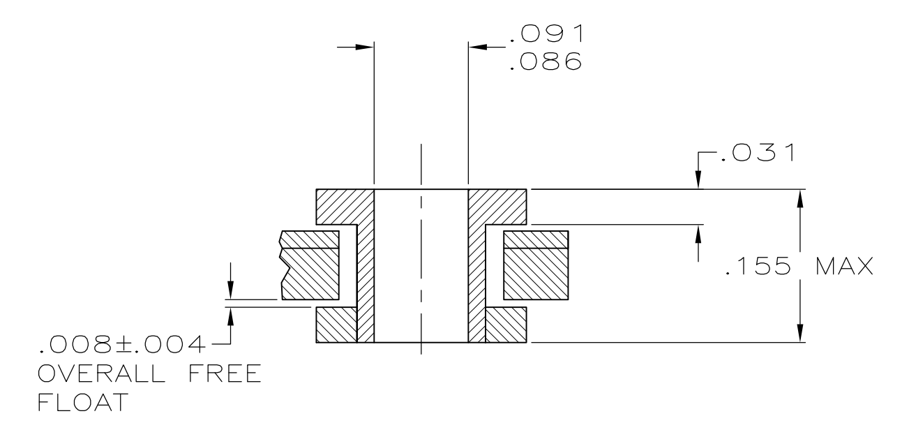
DUAL MOUNT FLOATING BUSHING SCALE 8:1
