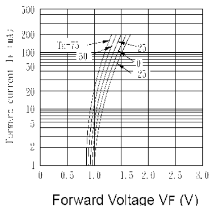
Fig.6 Forward Current vs. Forward Voltage
