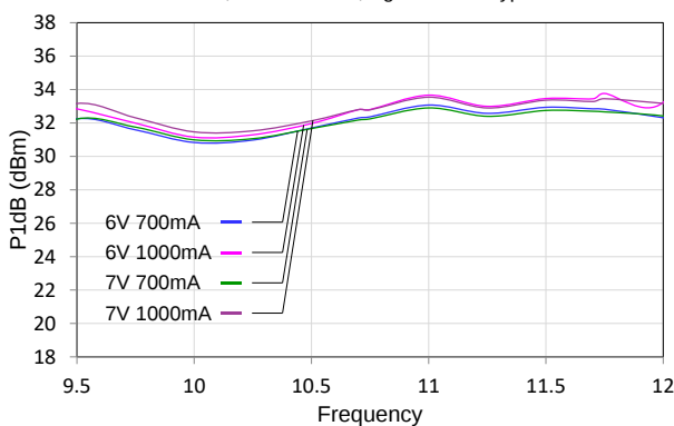
P1dB vs. Frequency vs. Bias (Vd1 and Vd2) Vd3 = 28 V, Id3 = 260 mA, Vg3 = -2.6 V Typical
