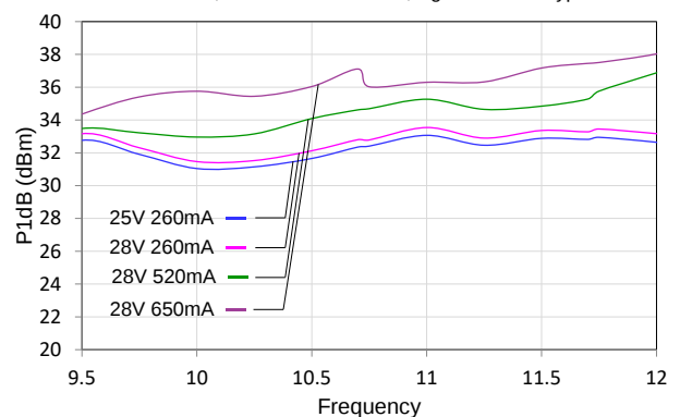
P1dB vs. Frequency vs. Bias (Vd3) Vd1 = Vd2 = 7 V, Id1 + Id2 = 1000 mA, Vg12 = -0.7 V Typical
