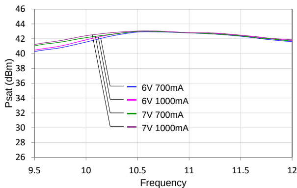
Psat vs. Frequency vs. Bias (Vd1 and Vd2) Vd3 = 28 V, Id3 = 260 mA, Vg3 = -2.6 V Typical
