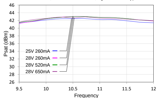
Psat vs. Frequency vs. Bias (Vd3) Vd1 = Vd2 = 7 V, Id1 + Id2 = 1000 mA, Vg12 = -0.7 V Typical
