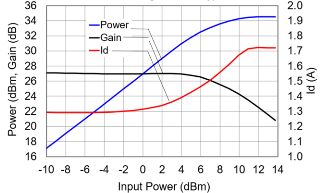
Power, Gain, I_d vs. Input Power @ 14 GHz
