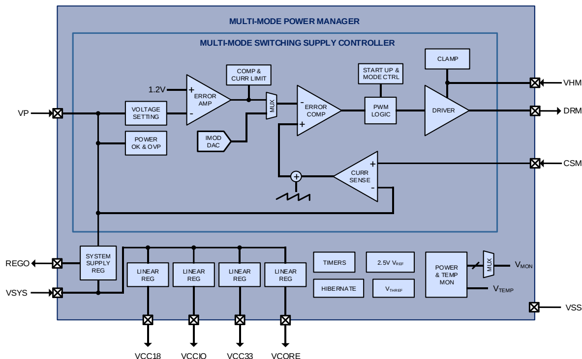
Figure 11-1 MMPM Block Diagram
