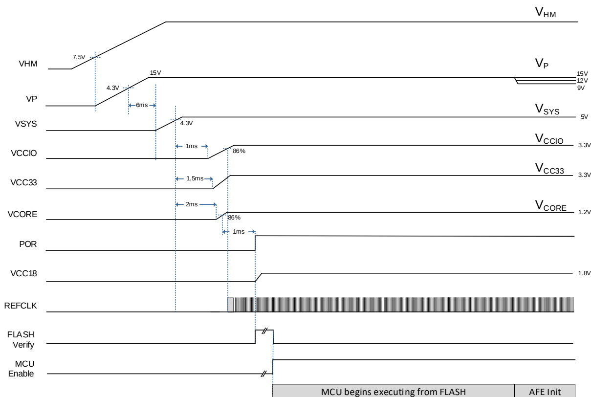
Figure 11-6 Power-Up Sequence
