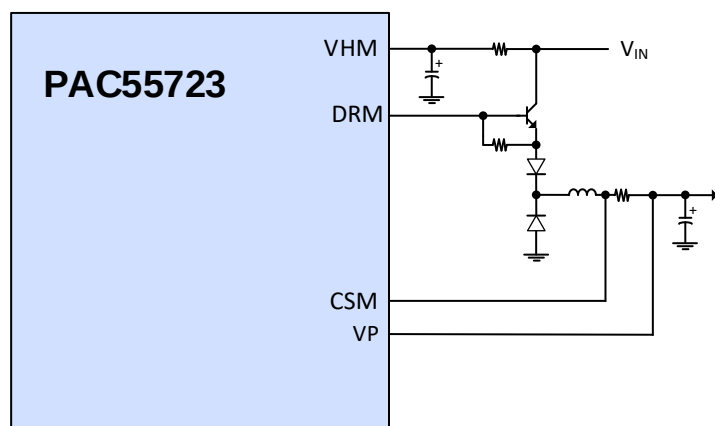
Figure 11-2 Buck Mode
