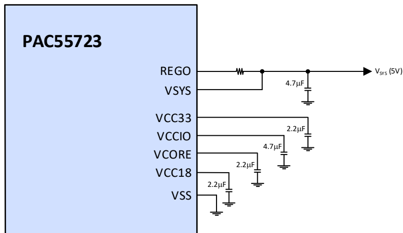
Figure 11-5 Linear Regulators
