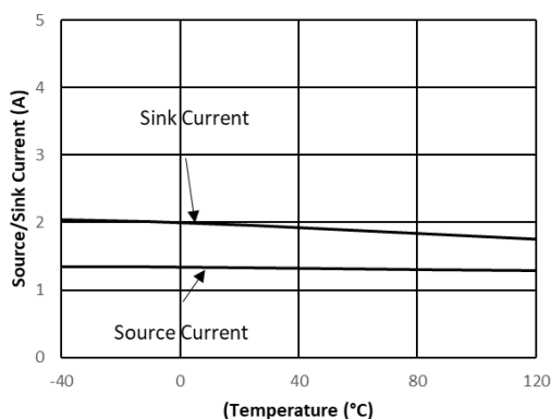
Low-Side Gate Driver (DRLx) Source/Sink Current vs. Temperature
