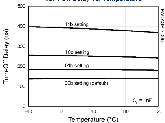
Low-Side Gate Driver (DRLx) Turn-Off Delay vs. Temperature
