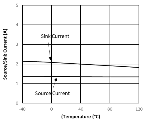
High-Side Gate Driver (DRHx) Source/Sink Current vs. Temperature
