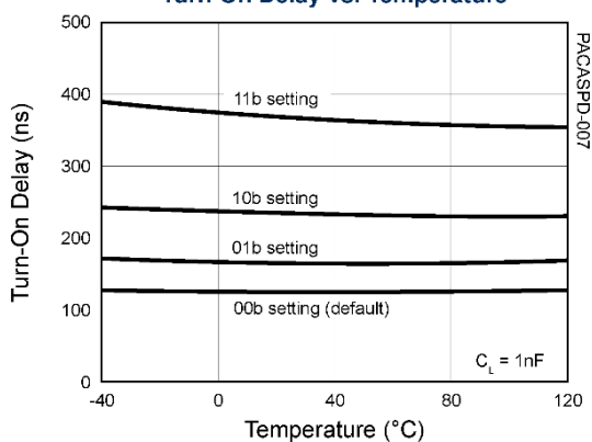
Low-Side Gate Driver (DRLx) Turn-On Delay vs. Temperature
