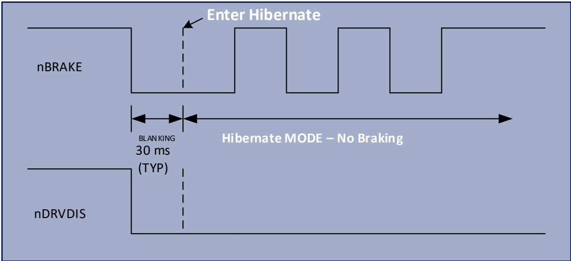
Figure 12-8 Entering Hibernate Mode (PAC55713 only)
