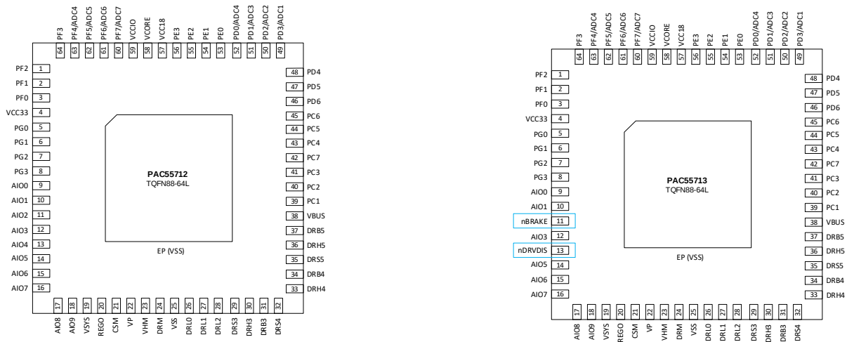
Figure 8-3 PAC55712 and PAC55713 Function Differences (pin comparison)
