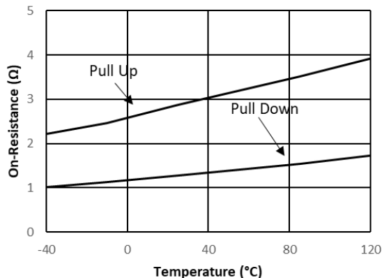
Low-Side Gate Driver (DRLx) On Resistance vs. Temperature
