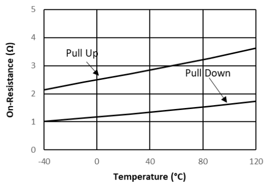
High-Side Gate Driver (DRHx) On Resistance vs. Temperature
