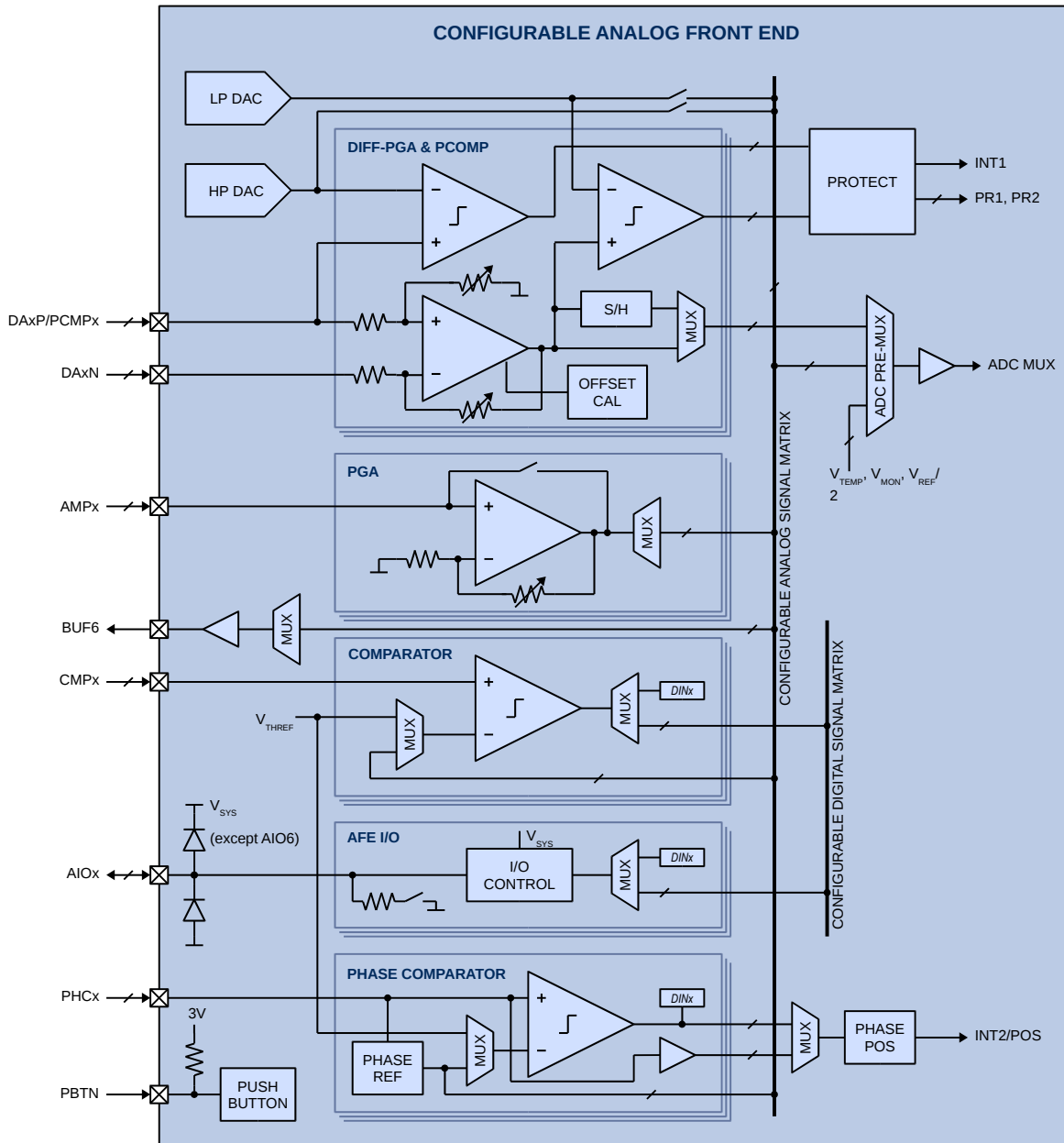
Figure 11-1 PAC52422 Configurable Analog Front End
