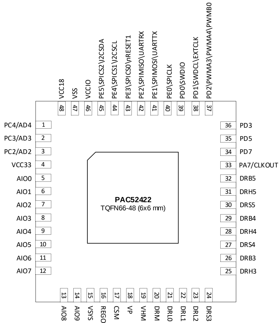
Figure 8-1 PAC52422 Pin Configuration (TQFN66-48 Package)
