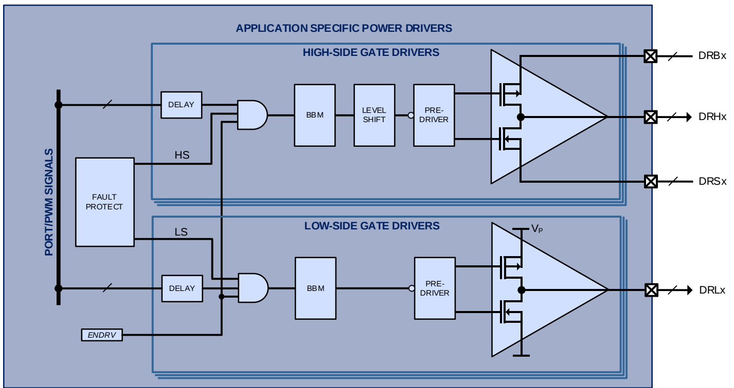
Figure 12-1 PAC52422 Application Specific Power Drivers
