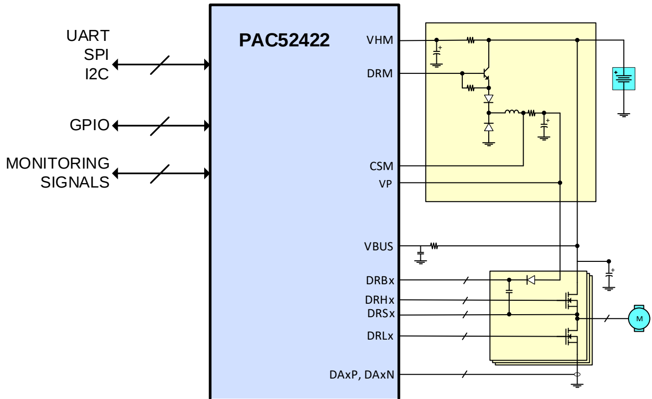
Figure 21-1 3-Phase Motor Drive Using PAC52422 (Simplified Diagram)
