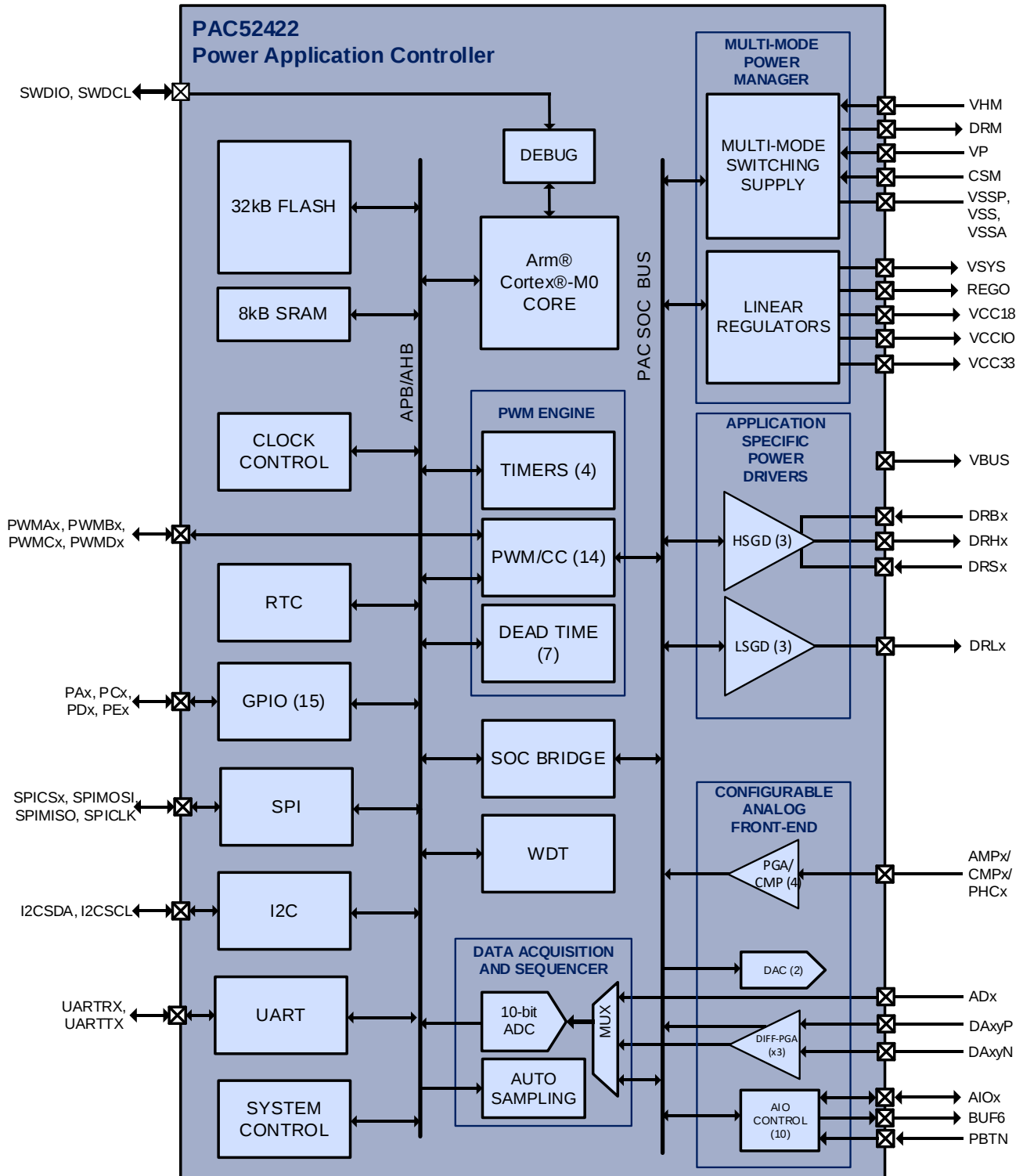
Figure 7-1 PAC52422 Architectural Block Diagram
