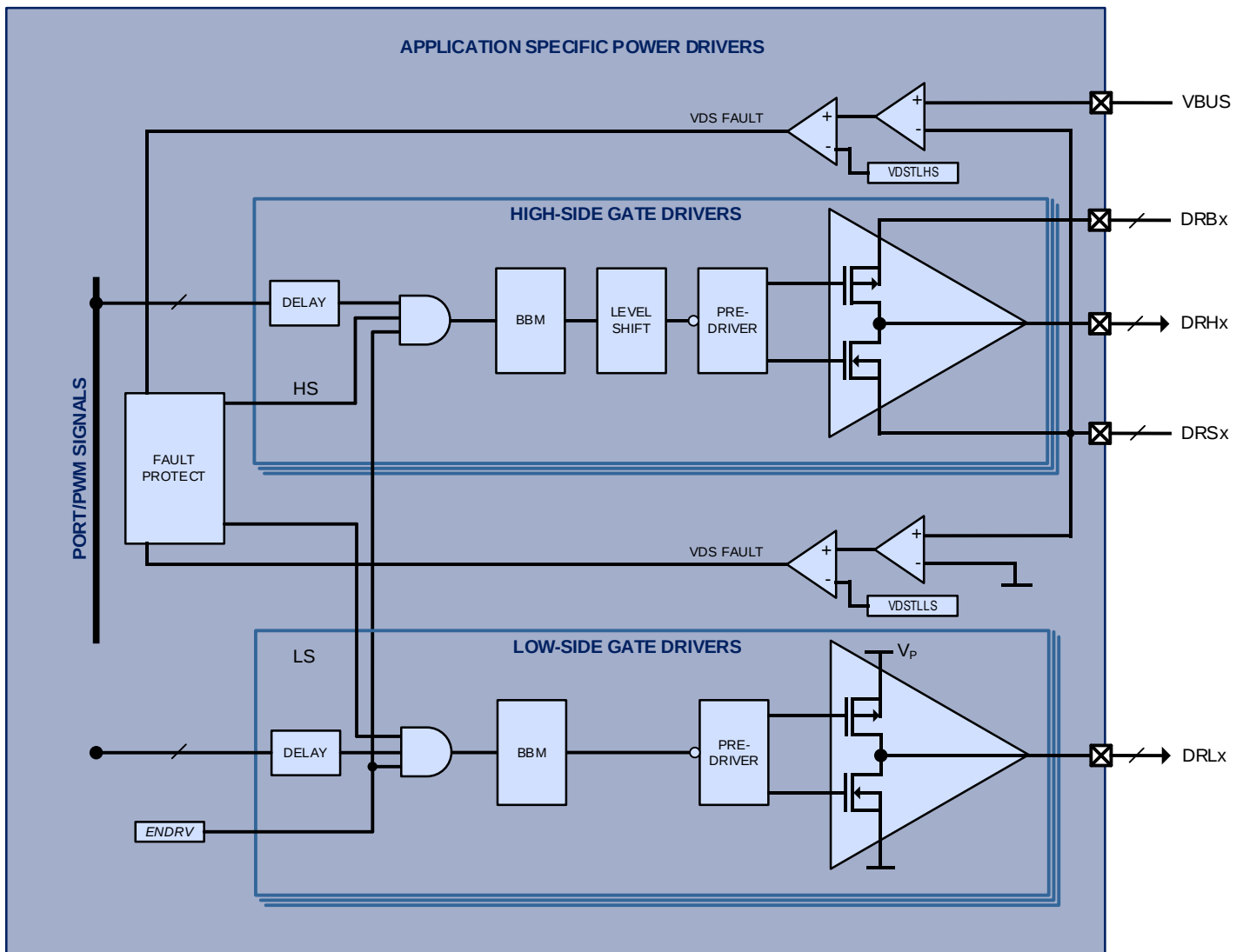
Figure 12-1 PAC52410 Application Specific Power Drivers
