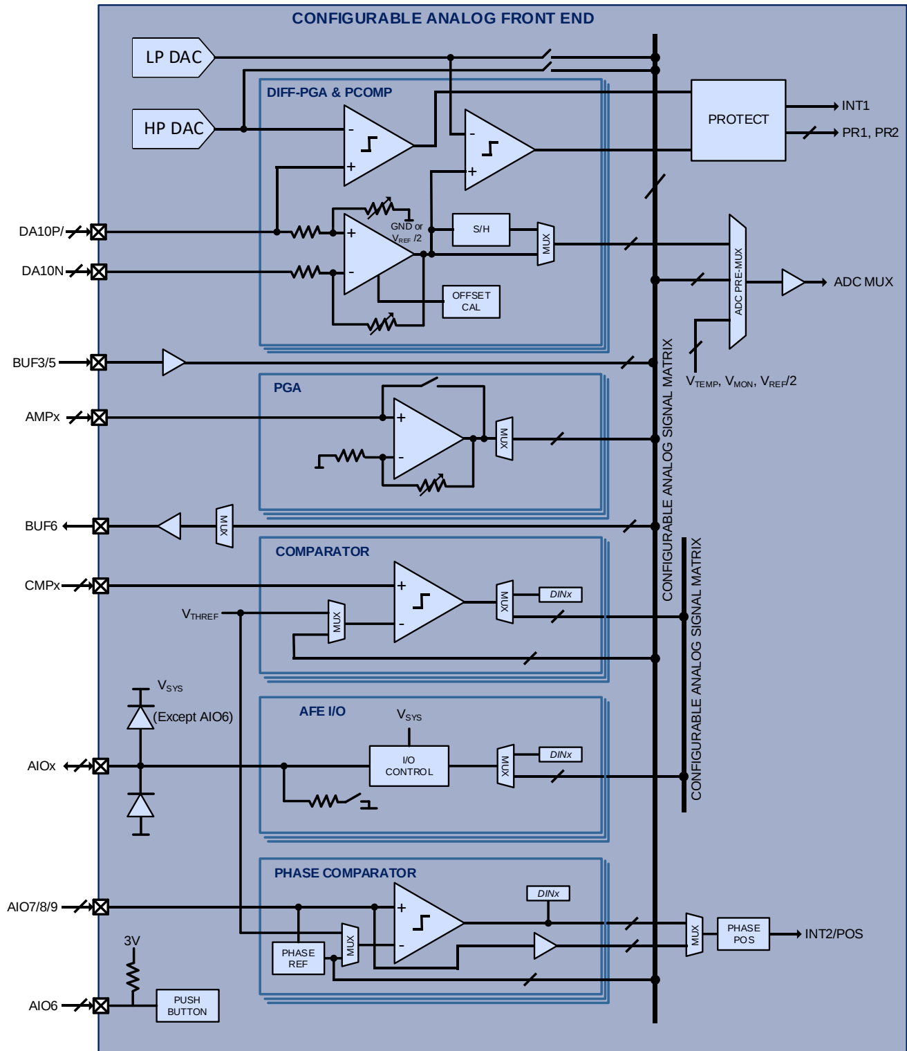
Figure 11-2 PAC52411 Configurable Analog Front End
