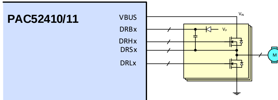
Figure 12-3 Typical Gate Driver Connections
