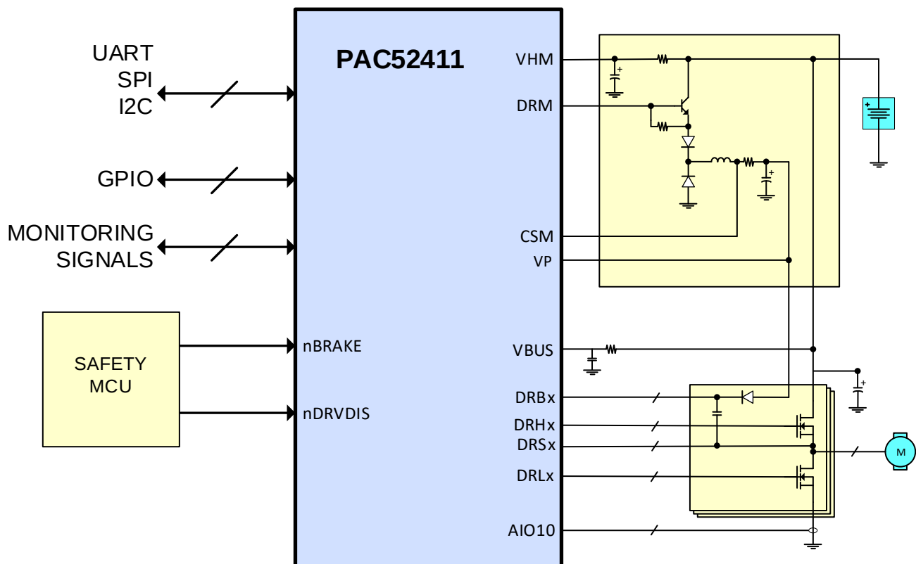
Figure 21-2 3-Phase Motor Drive Using PAC52411 and Safety MCU (Simplified Diagram)
