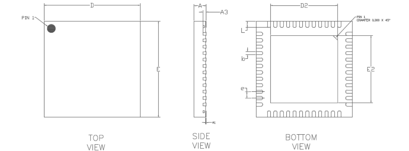
Figure 22-1 TQFN66-48 Package Outline and Dimensions
