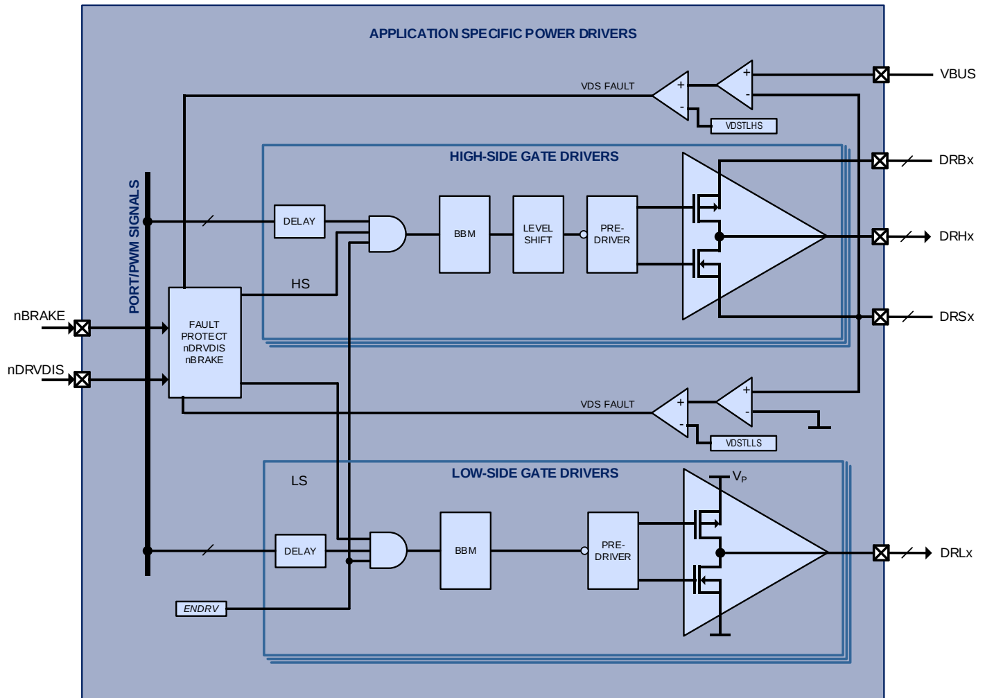
Figure 12-2 PAC52411 Application Specific Power Drivers
