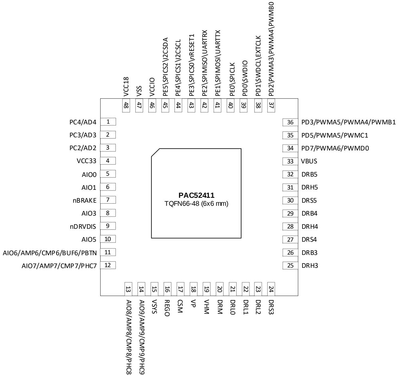
Figure 8-2 PAC52411 Pin Configuration (TQFN66-48 Package)
