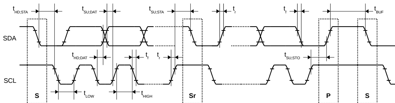
Figure 18-2 I 2 C Timing Diagram
