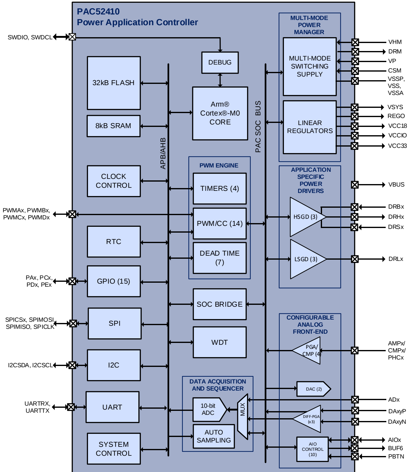
Figure 7-1 PAC52410 Architectural Block Diagram
