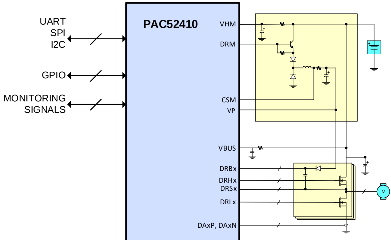
Figure 21-1 3-Phase Motor Drive Using PAC52410/11 (Simplified Diagram)
