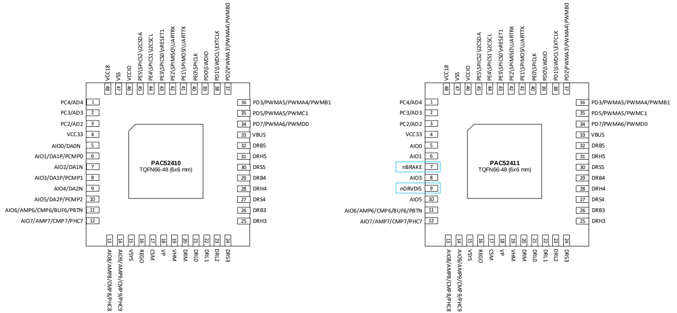
Figure 8-3 PAC52410 and PAC52411 Function Differences (pin comparison)
