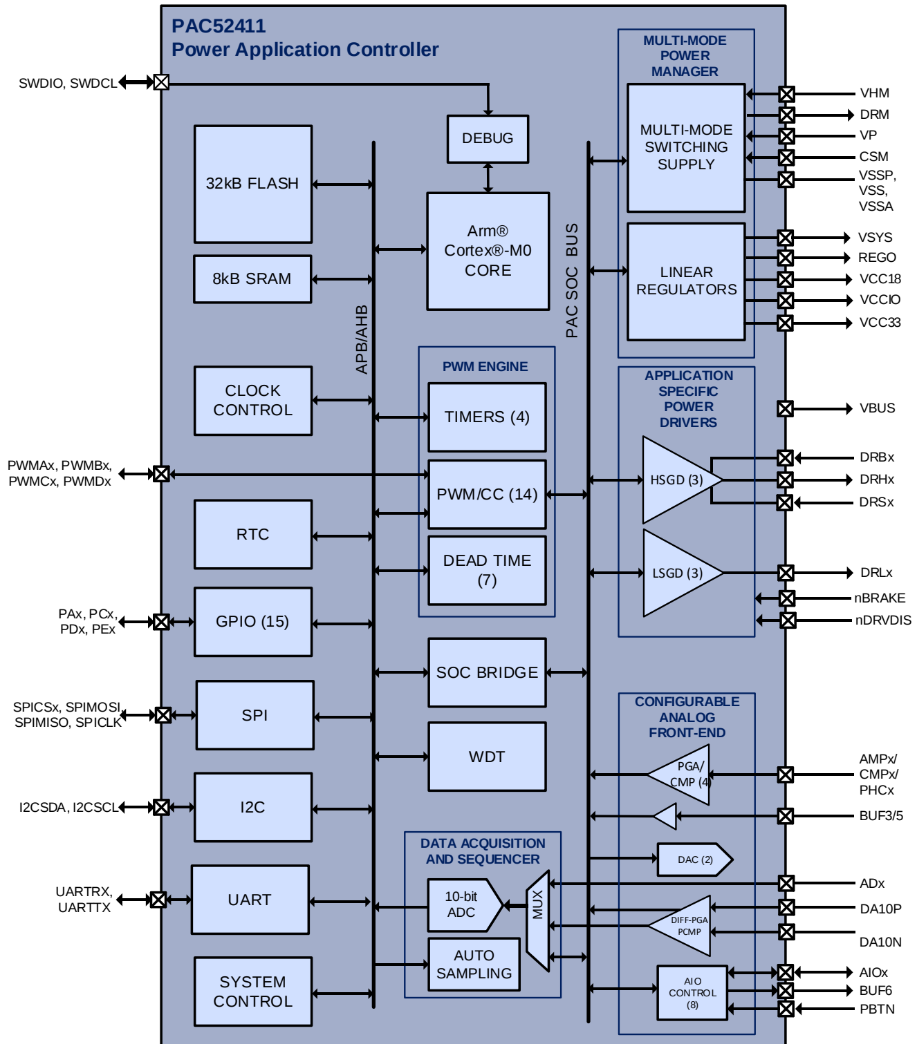
Figure 7-2 PAC52411 Architectural Block Diagram
