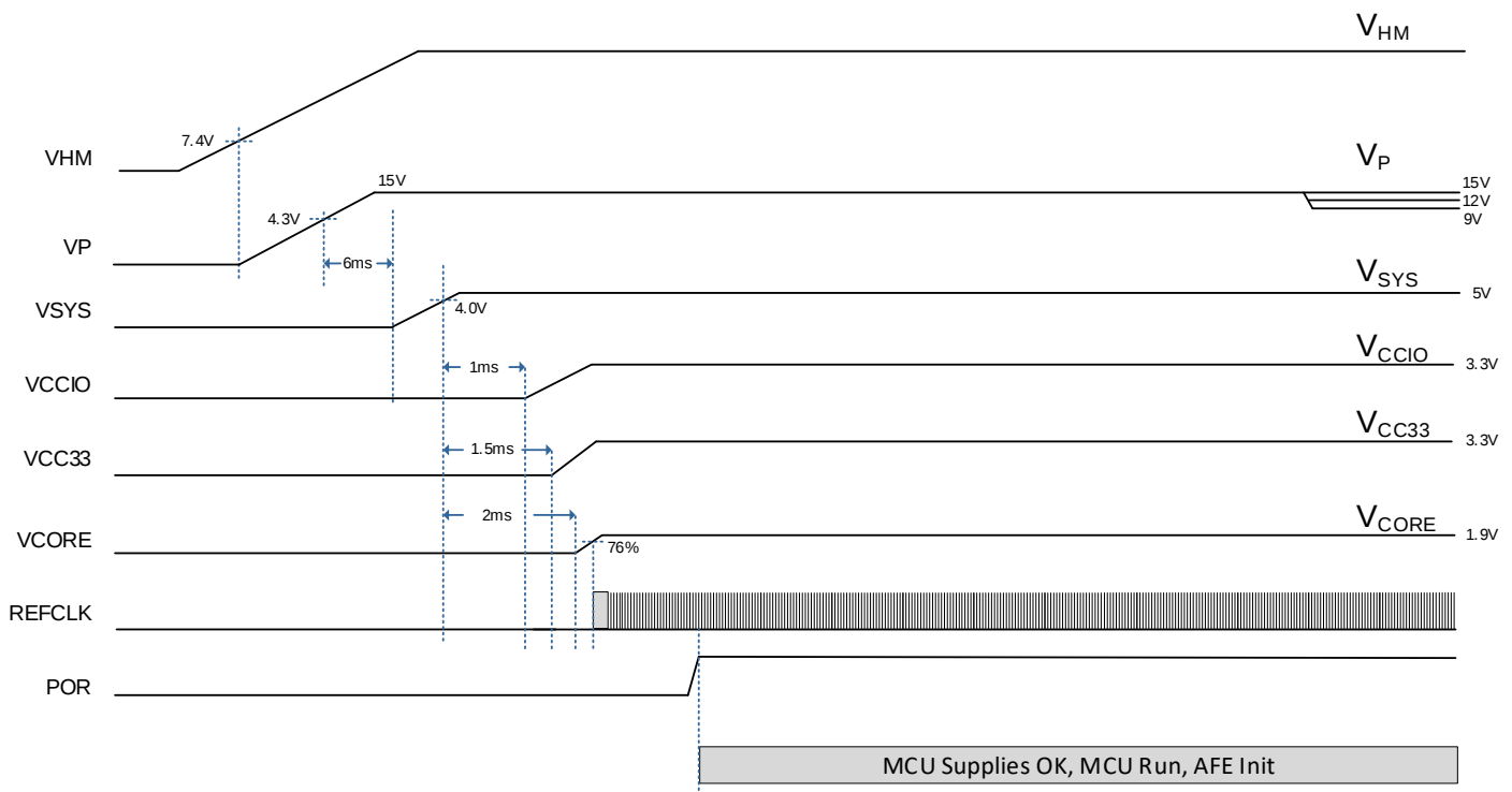
Figure 10-6 Power Up Sequence
