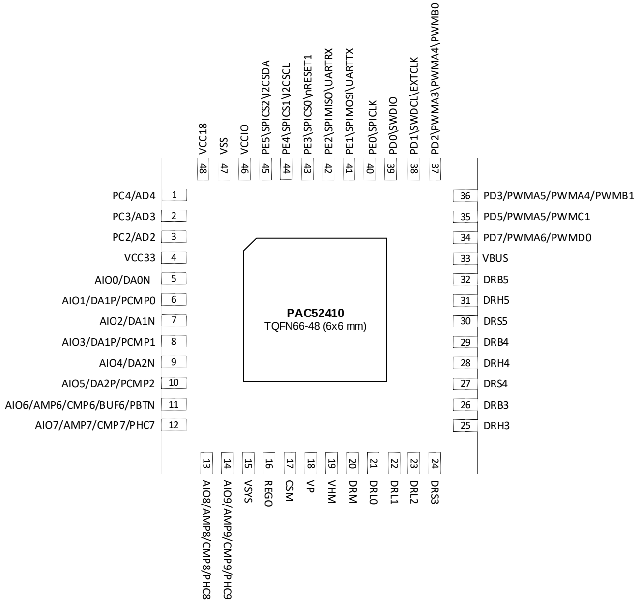
Figure 8-1 PAC52410 Pin Configuration (TQFN66-48 Package)
