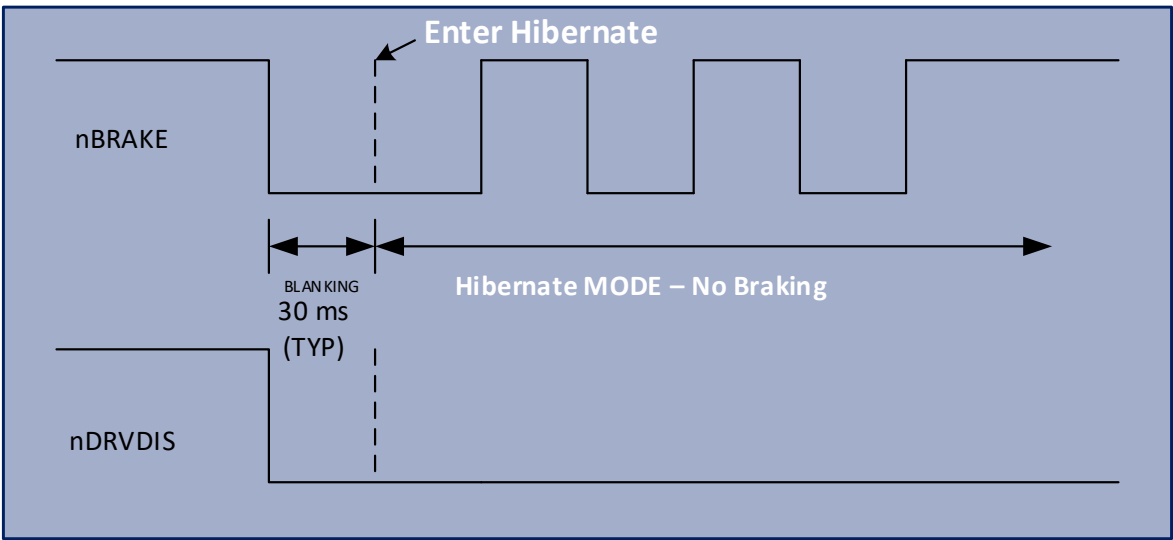
Figure 12-8 Entering Hibernate Mode (PAC52411 only)
