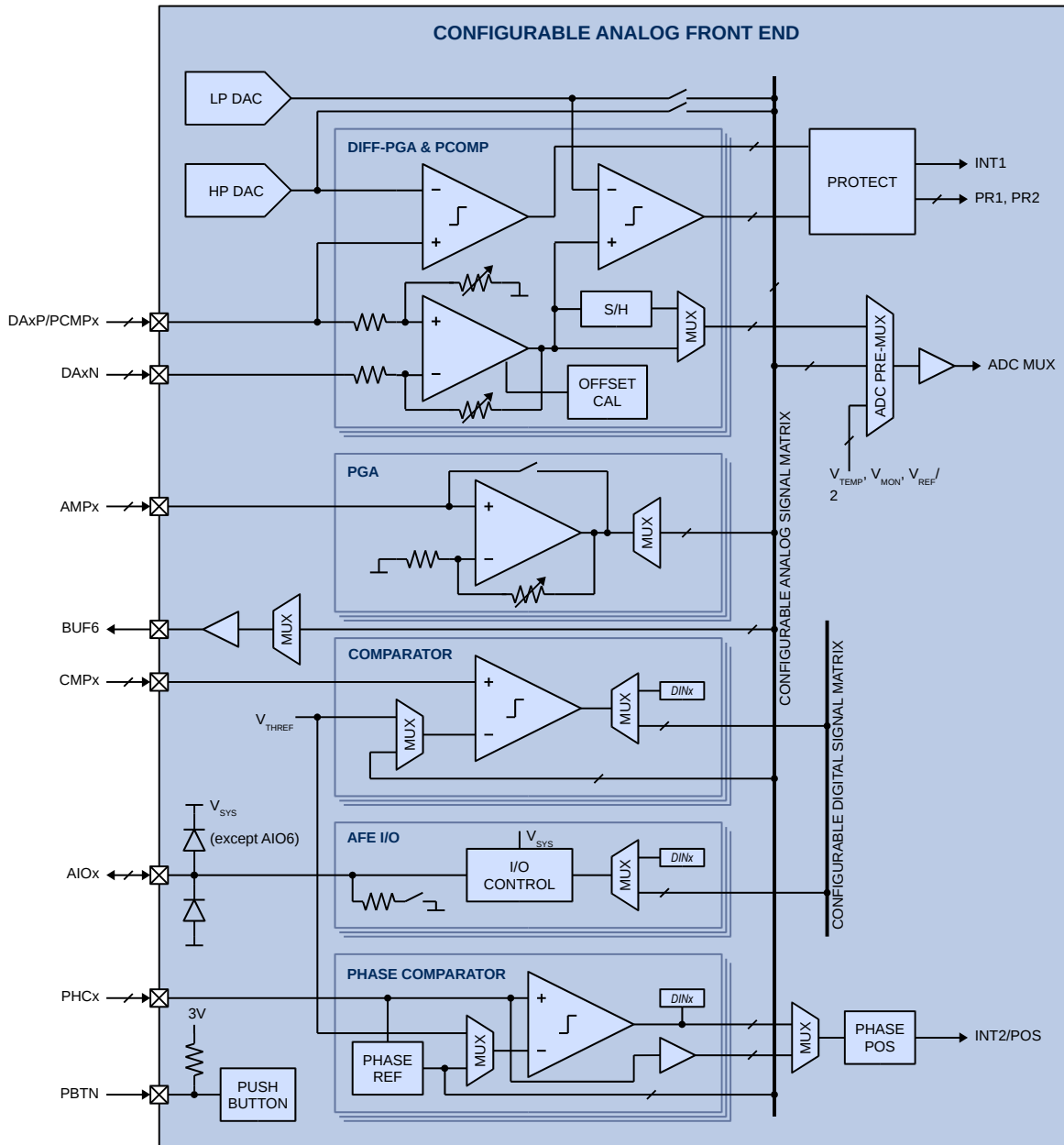
Figure 11-1 PAC52410 Configurable Analog Front End
