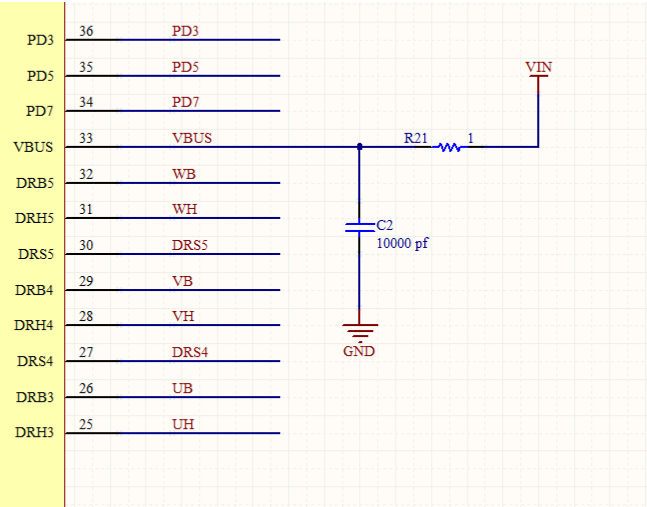
Figure 9-2 VBUS RC Filter Connections
