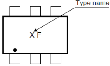
Fig. 9.6 Marking RN1906FE
