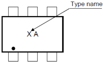
Fig. 9.1 Marking RN1901FE
