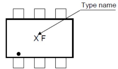
Fig. 9.6 Marking RN1906FE
