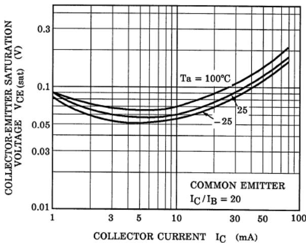
Fig. 10.21 RN1903FE V_{CE(sat)}-I_C
