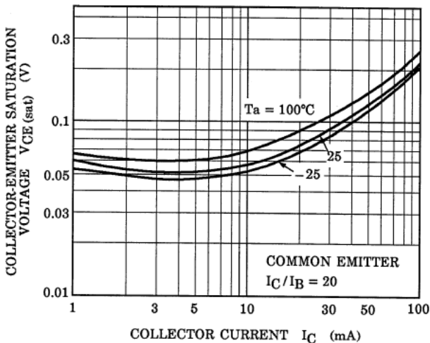
Fig. 10.23 RN1905FE V_{CE(sat)}-I_C
