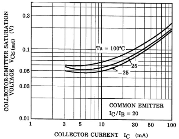
Fig. 10.20 RN1902FE V_{CE(sat)}-I_C
