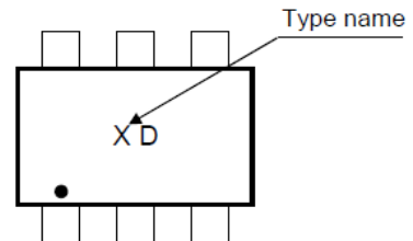
Fig. 9.4 Marking RN1904FE
