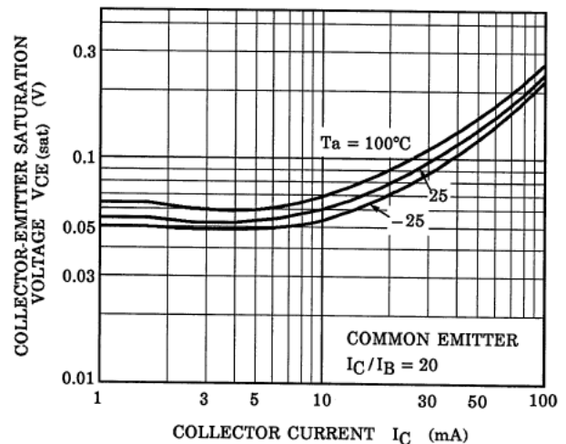
Fig. 10.24 RN1906FE V_{CE(sat)}-I_C
