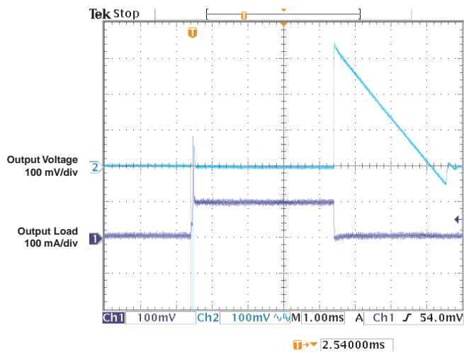
LOAD TRANSIENT RESPONSE vs TIME ( V_{OUT} = 5\text{ V} , C_L = 1\text{ }\mu\text{F} )
