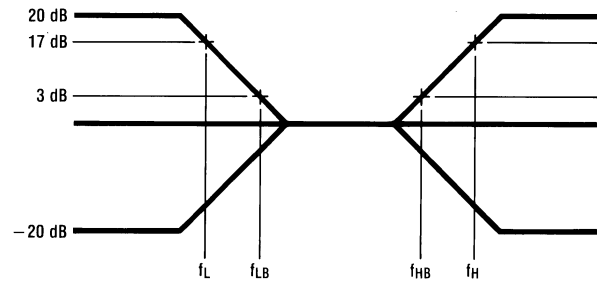
Figure 92. Tone Control
