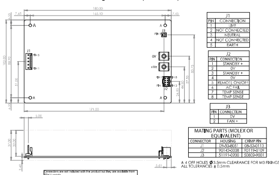
Outline & Connection Drawings - Class I (with earth)
