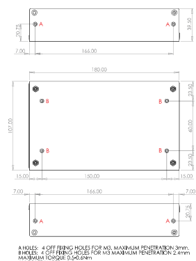
STANDARD CHASSIS
