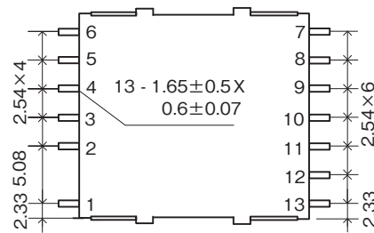
Rear surface
