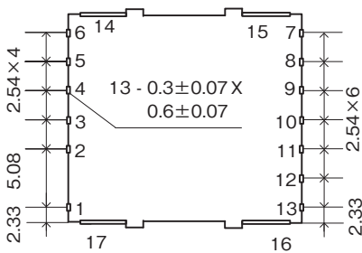
Rear surface
