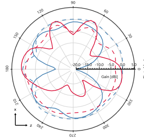
Gain (Total) - \phi = 0^\circ deg - 2100 MHz [Plane XZ]
