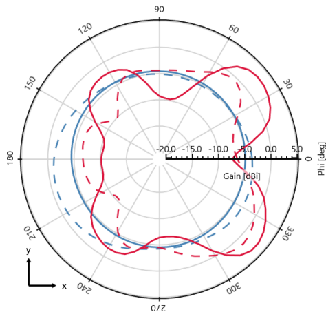
Gain (Total) - \theta = 90^\circ deg - 960 MHz [Plane XY]
