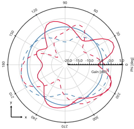
Gain (Total) - \theta = 90^\circ deg - 1700 MHz [Plane XY]
