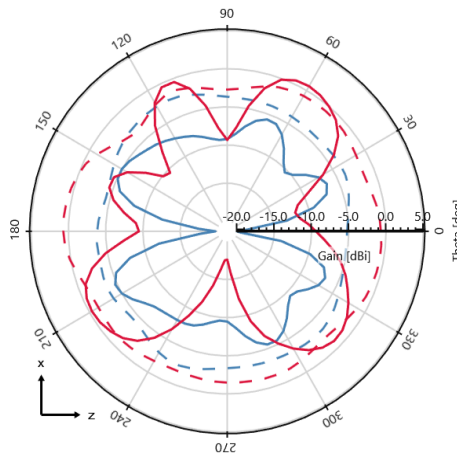
Gain (Total) - \phi = 0 deg - 1400 MHz [Plane XZ]
