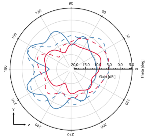
Gain (Total) - \phi = 90^\circ deg - 700 MHz [Plane YZ]
