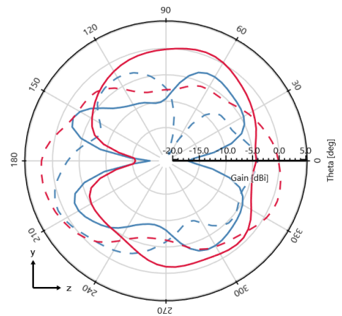
Gain (Total) - \phi = 90 deg - 1500 MHz [Plane YZ]
