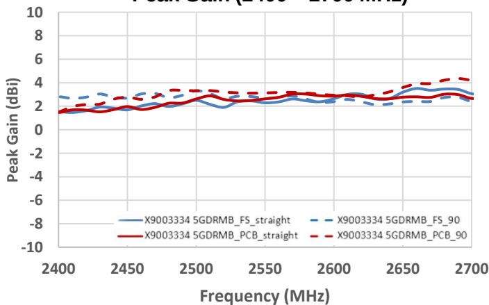
Peak Gain (2400 – 2700 MHz)
