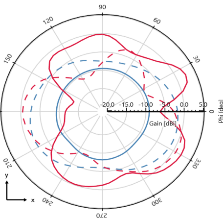
Gain (Total) - \theta = 90 deg - 1500 MHz [Plane XY]
