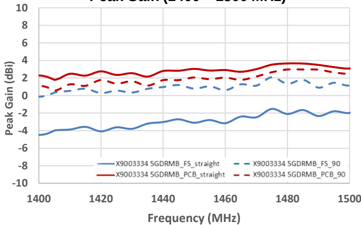
Peak Gain (1400 – 1500 MHz)
