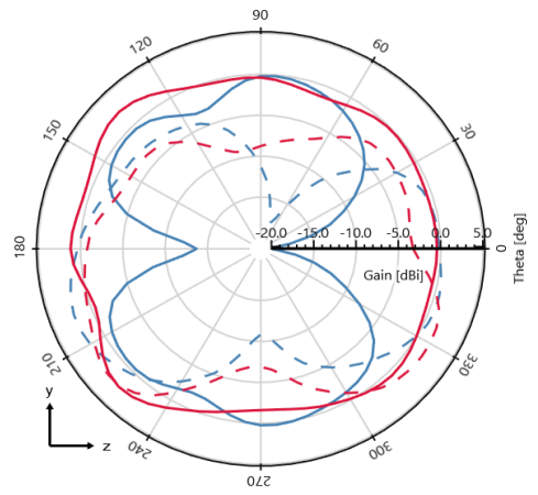
Gain (Total) - \phi = 90^\circ deg - 2100 MHz [Plane YZ]
