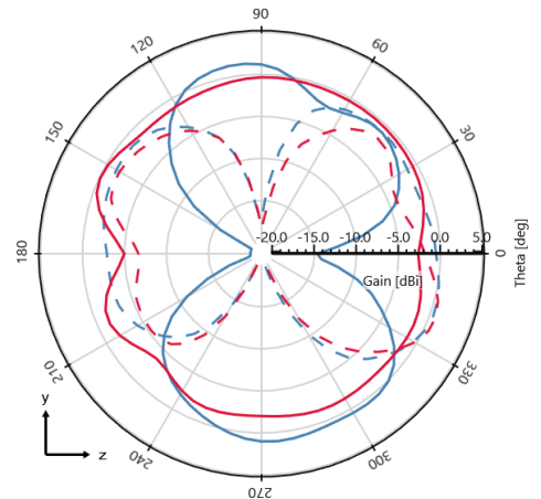
Gain (Total) - \phi = 90 deg - 3300 MHz [Plane YZ]
