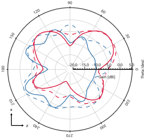
Gain (Total) - \phi = 0^\circ deg - 700 MHz [Plane XZ]
