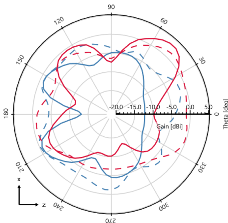
Gain (Total) - \phi = 0^\circ deg - 960 MHz [Plane XZ]
