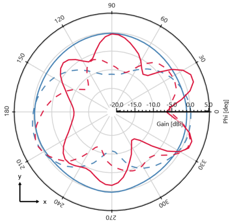
Gain (Total) - \theta = 90^\circ deg - 2100 MHz [Plane XY]
