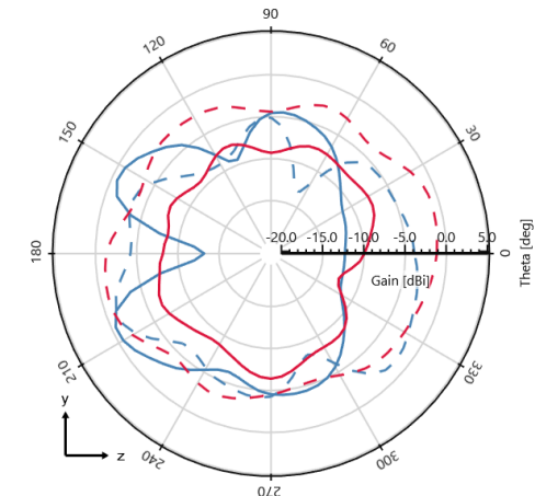
Gain (Total) - \phi = 90^\circ deg - 960 MHz [Plane YZ]
