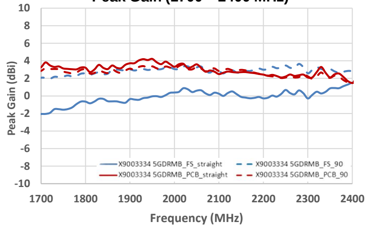
Peak Gain (1700 – 2400 MHz)
