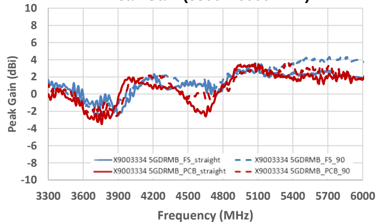
Peak Gain (3300 – 6000 MHz)
