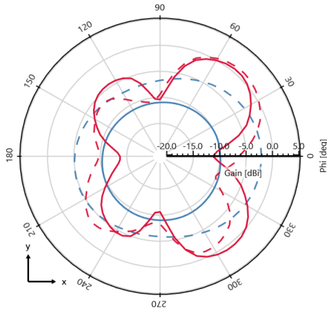
Gain (Total) - \theta = 90^\circ deg - 700 MHz [Plane XY]
