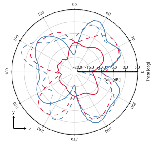
Gain (Total) - \phi = 90 deg - 5000 MHz [Plane YZ]
