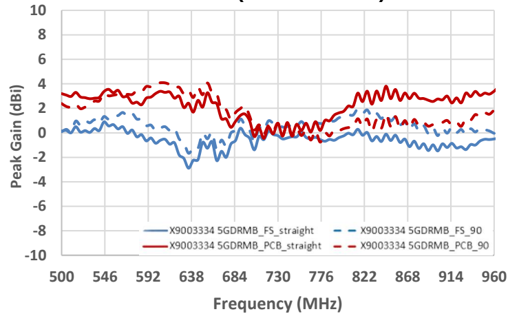
Peak Gain (500 – 960 MHz)
