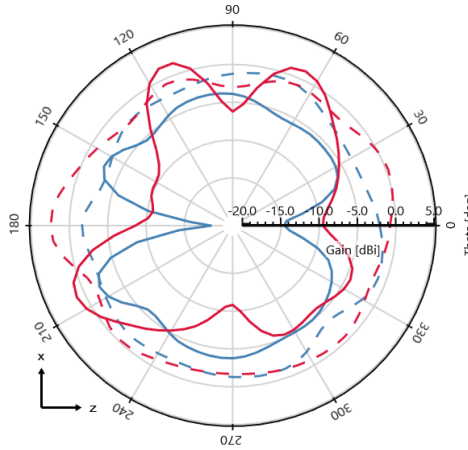
Gain (Total) - \phi = 0^\circ deg - 1700 MHz [Plane XZ]
