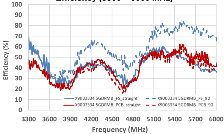
Efficiency (3300 – 6000 MHz)
