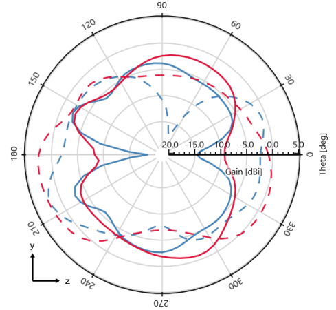
Gain (Total) - \phi = 90^\circ deg - 1700 MHz [Plane YZ]
