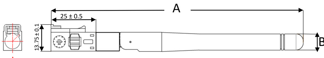
Straight View
