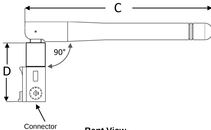
Bent View
