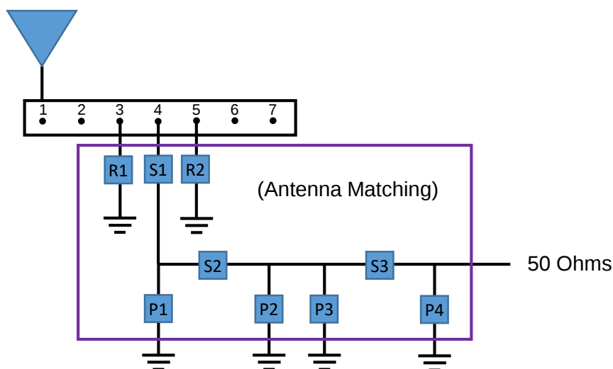
(Antenna Matching): pads are directly inline with the antenna feed trace.
