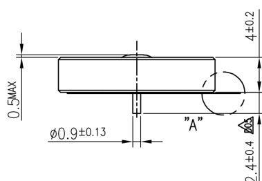
003 Side View
