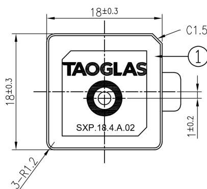
001 003 Front View
