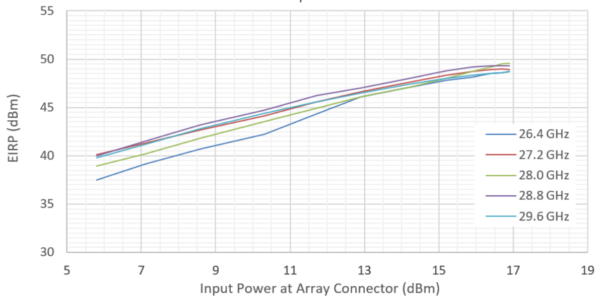
KHA16.24C Array EIRP H-pol
