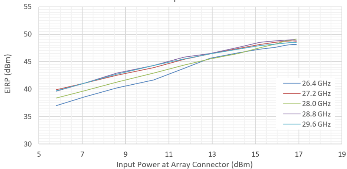
KHA16.24C Array EIRP V-pol
