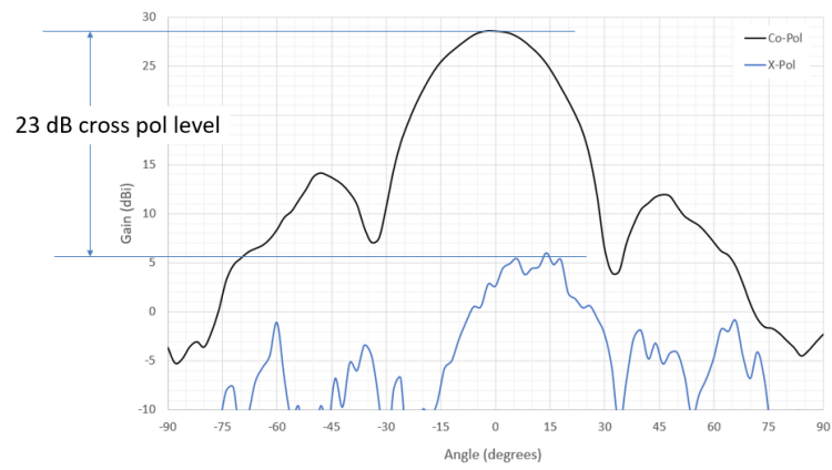
Boresight radiation pattern, Co and cross-pol, 28.0 GHz, H-pol
