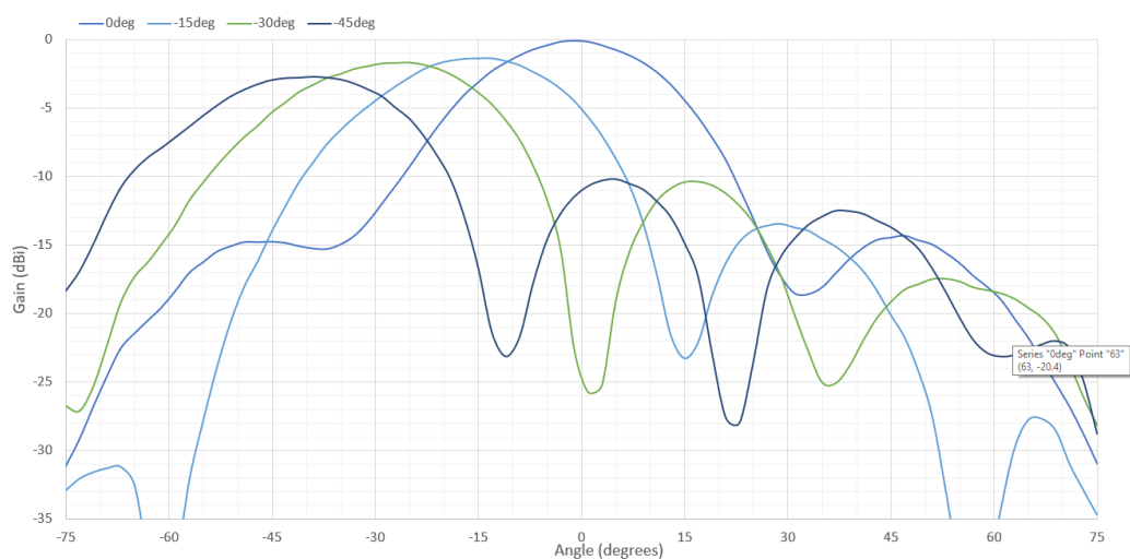
26.8GHz Azimuth Scan, V-pol
