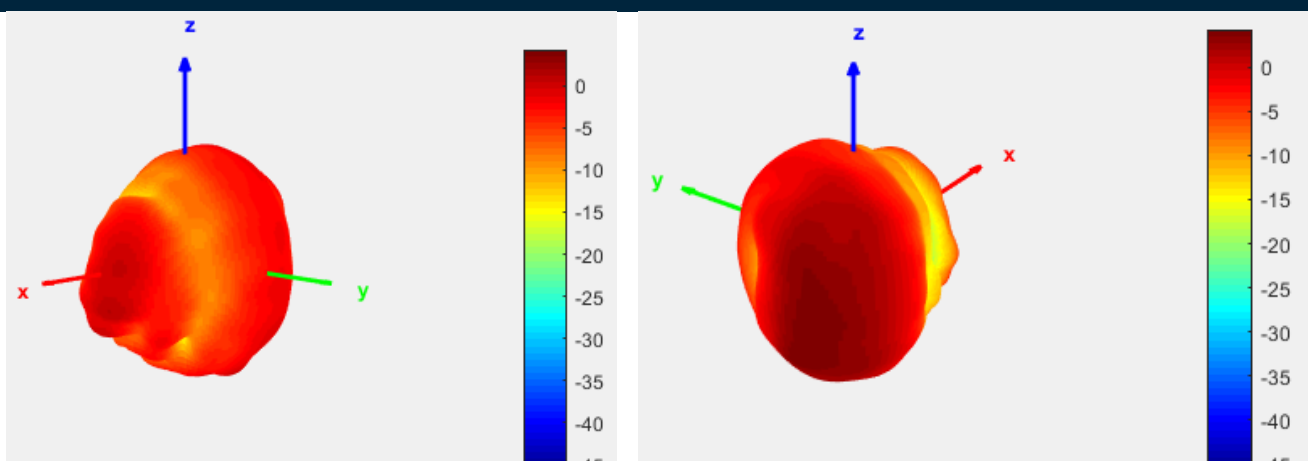
Radiation Pattern at 7.5GHz
