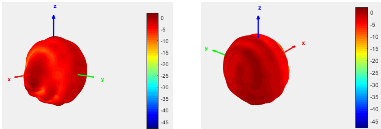
Radiation Pattern at 7.5GHz
