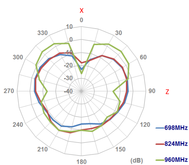
XZ Plane
