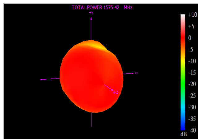
1575.42MHz
