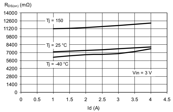
Figure 19. Static drain source on-resistance vs drain current (3 pin)
