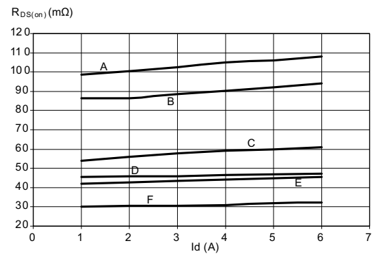
Figure 21. Static drain source on-resistance vs drain current
