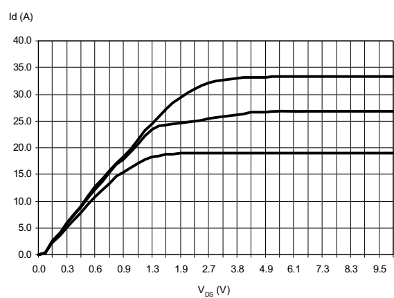
Figure 23. Output characteristics
