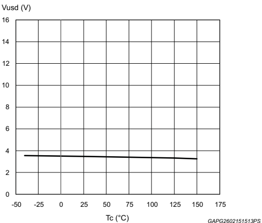
Figure 14. Undervoltage shutdown
