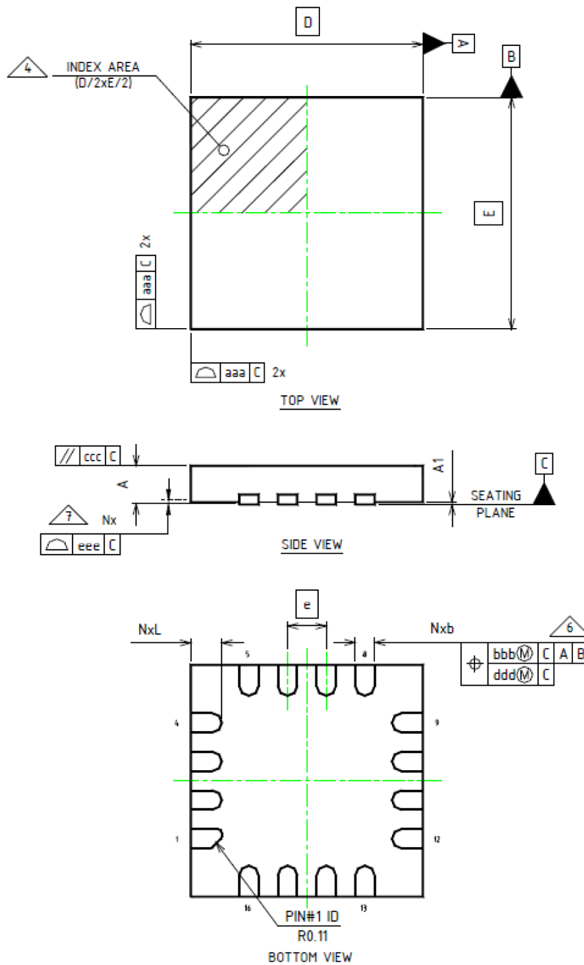
Figure 11. QFN16 (3x3x0.55) package outline
