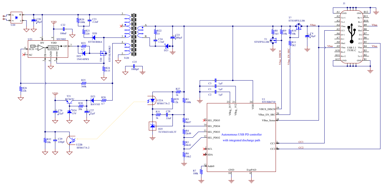
Figure 8. Flyback topology
