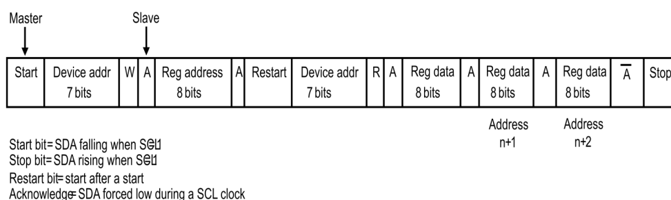
Figure 4. Read operation
