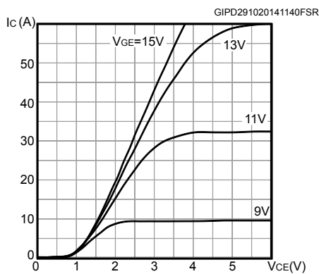
Figure 3. Output characteristics ( T_J = 25^\circ\text{C} )
