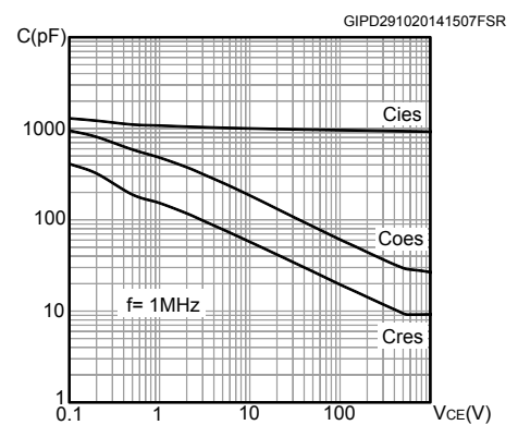
Figure 12. Capacitance variations
