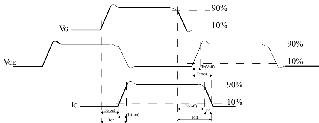
Figure 24. Switching waveform
