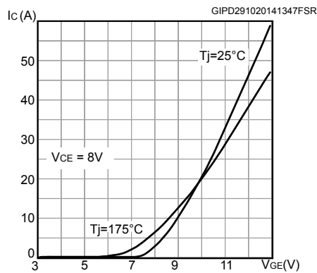
Figure 9. Transfer characteristics
