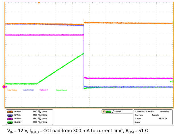
Figure 30. Overcurrent protection during operation (latched version)
