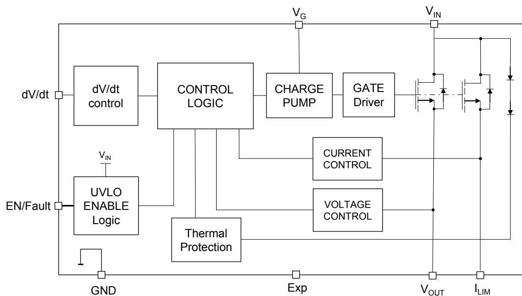
Figure 1. Block diagram
