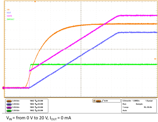
Figure 26. Startup into voltage clamp
