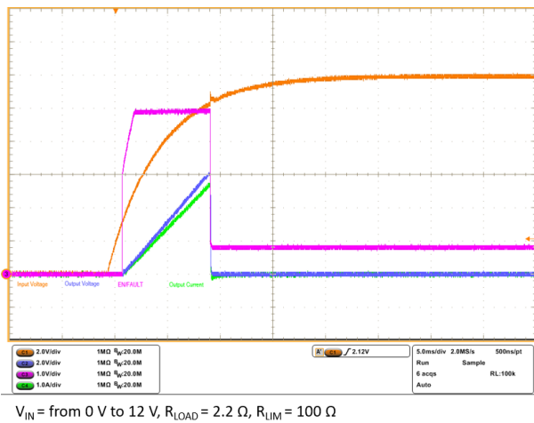
Figure 29. Startup into overload
