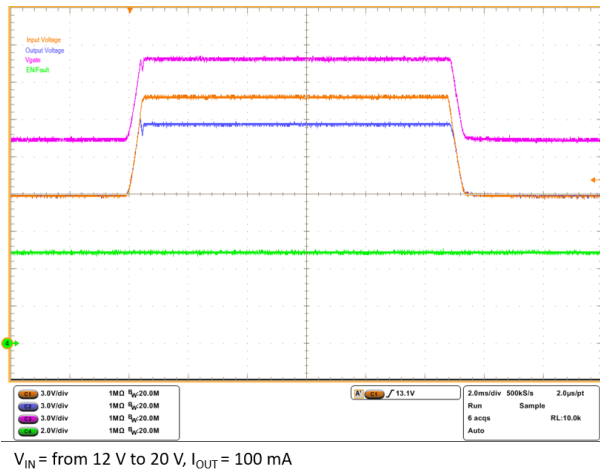
Figure 27. Voltage clamp during operation
