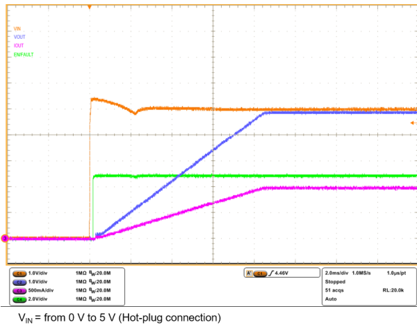
Figure 25. Startup with R_{LOAD} = 5\ \Omega
