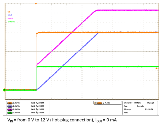
Figure 24. Startup with no load
