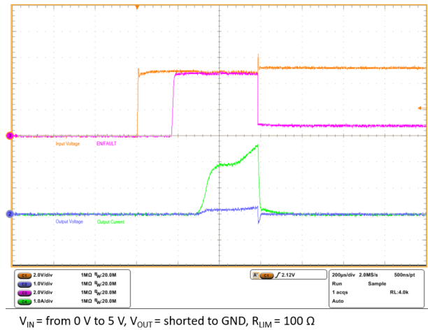
Figure 28. Start-up into output short-circuit
