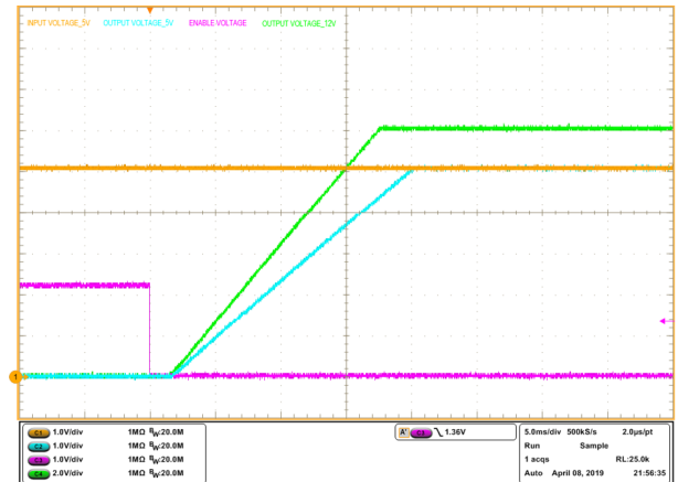
Figure 8. Start-up by EN, no load
