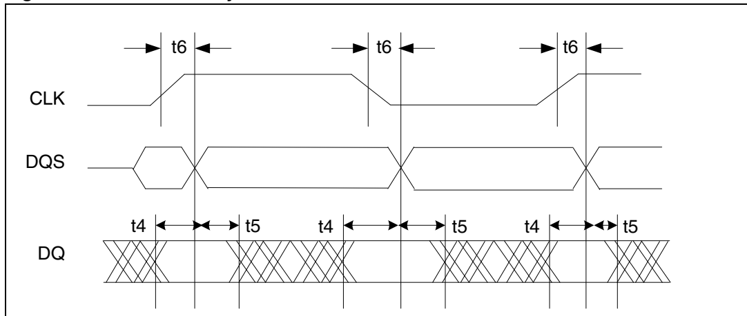
Figure 11. DDR2 Write cycle path
