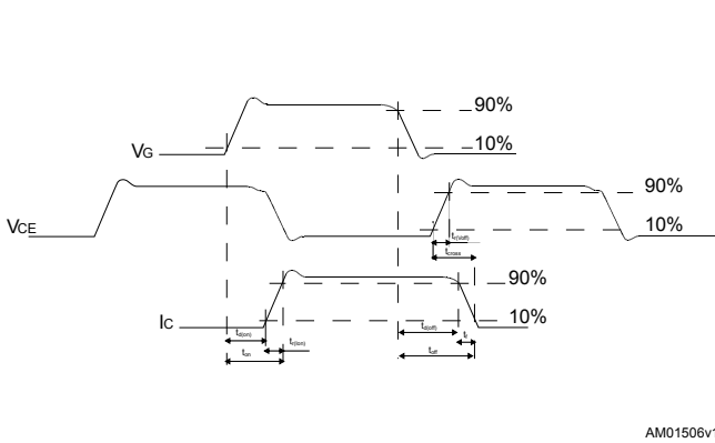
Figure 28. Switching waveform
