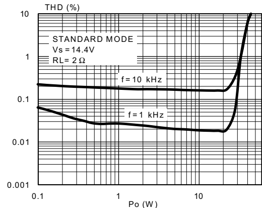
Figure 9. Distortion vs. output power (2 Ω, STD)
