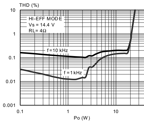
Figure 8. Distortion vs. output power (4 Ω, HI-EFF)
