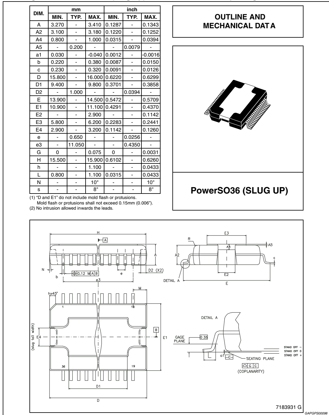
Figure 40. PowerSO36 (slug up) mechanical data and package dimensions
